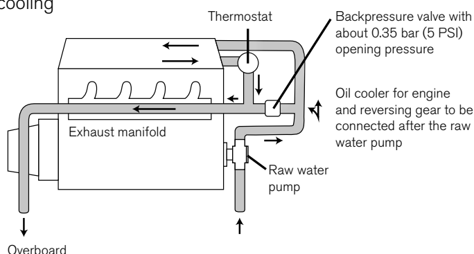
Direct cooling
